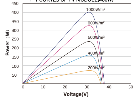
P-V CURVES OF PV MODULE(400W)
